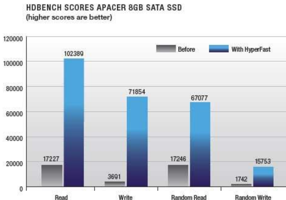
Figure 1: Performance Benefits from HyperFast
